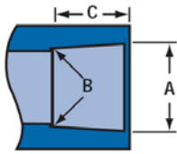
STANDARD SCHEDULE 80 SOCKET DIMENSIONS ASTM D 2467
